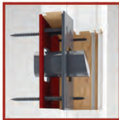
Security plates for the double-anchoring deadbolt lock
